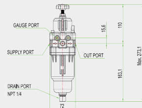
YT-220/YT-225 (Manual Drain / Auto. Drain)
