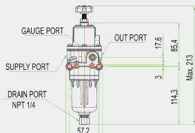
YT-200/YT-205 (Manual Drain / Auto. Drain)
