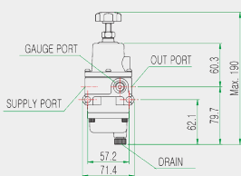
YT-200/YT-205 (Manual Drain / Auto. Drain)
